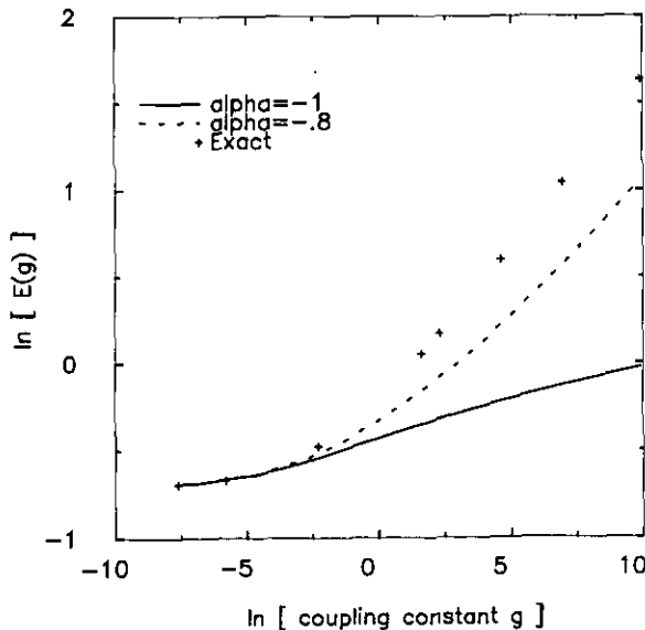
Figure 1. Octic oscillator ground state eigenvalue versus coupling constant g .
