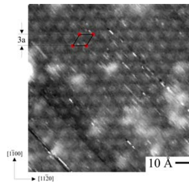
Figure 4: STM images of room temperature Cr deposited GaN(000-1) surface, 3×3 reconstruction image of the surface. [ V_s = -1V ; I_t =
