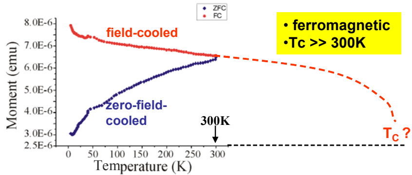
Fig. 5 SQUID result for thick CrGaN sample.
