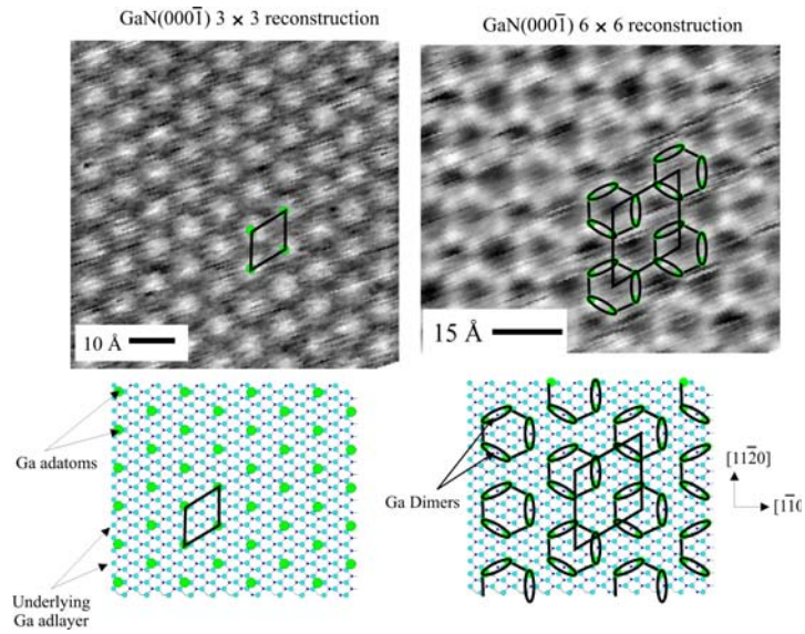
Figure 1 STM images of GaN(000-1) surface. a) 3×3 reconstruction image acquired at V_s = +1.5V and I_t = 0.08nA and b) 6×6 reconstruction image with schematic model superimposed on the STM image [ V_s = +2V ; I_t = 0.08nA ].
