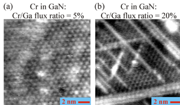
Figure 6 STM images of 5% Cr-doped GaN(000-1) surface, showing 3x3 reconstruction with apparent substitutional Cr atoms [ V_s = +1V ; I_t = 0.08nA ] STM images of 20% Cr-doped GaN(000-1) surface, showing Cr nanowires [ V_s = -1V ; I_t = 0.08nA ]
