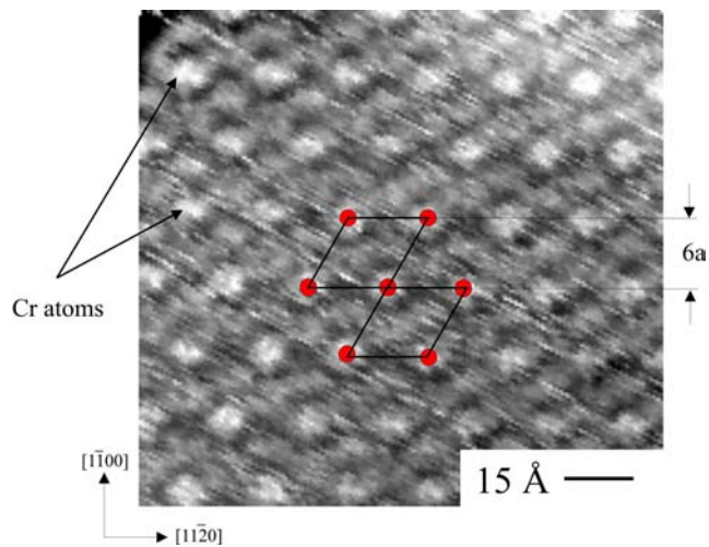
Figure 2 STM images of high temperature Cr deposited GaN(000-1) surface, 6×6 reconstruction image where Cr atoms are apparent in the image [ V_s = -1.5V ; I_t = 0.08nA ].
