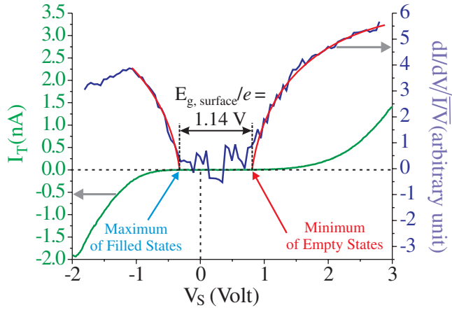
1 FIG. 3 (color). I_T vs V_S , averaged over 16 individual I - V spectra, acquired on the 4 \times 1 surface reconstruction (left y axis), and normalized conductance vs V_S (right y axis). Red curves are fits to the conduction and valence band DOS. Peaks inside the band gap are noise.
